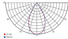
60° wide beam angle with optional 60° lens
