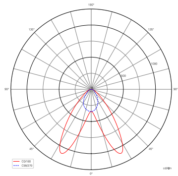
25°, double-sided asymmetrical
