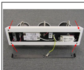
Figure 1 Remove the screws
