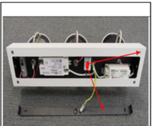
Figure 2 Remove the wires
